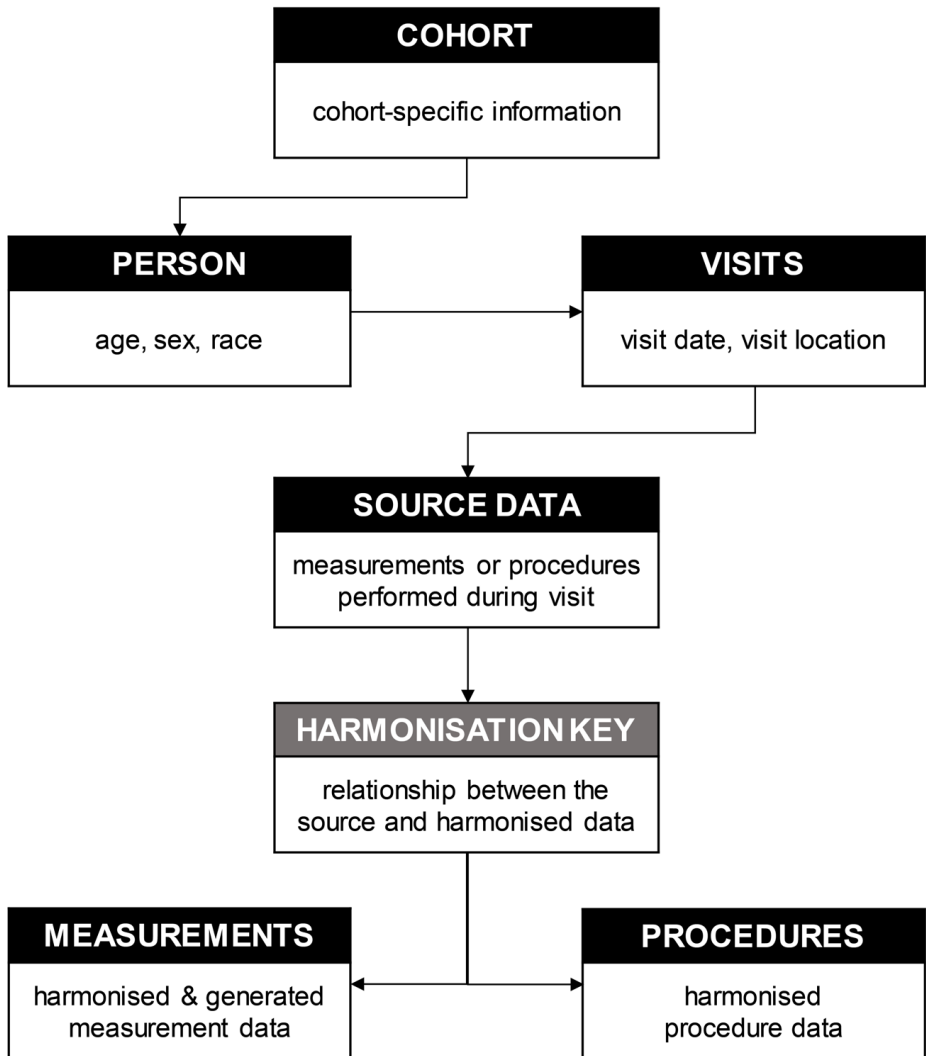
Figure 2: A simplified schema of the relational database used in the World COACH consortium.
